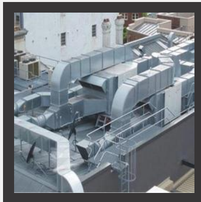
Exhaust Ducts
